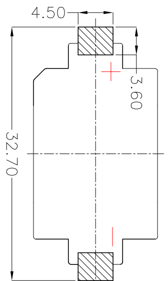
PCB Layout Diagram Top View
